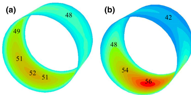
Fig. 7 Contours of temperature (°C) for a circumferential journal surface, b circumferential bearing surface for \varepsilon = 0.5 at N = 1,500 rpm
