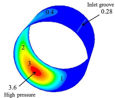
Fig. 5 Contours of pressure (MPa) for \varepsilon = 0.5 at N = 1,500 rpm
