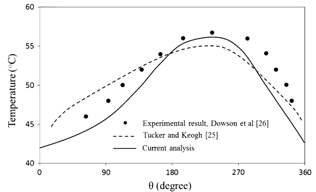
Fig. 9 Comparison of experimental result and current analysis for circumferential bearing bushing surface temperatures for \varepsilon = 0.5 at N = 1,500 rpm
