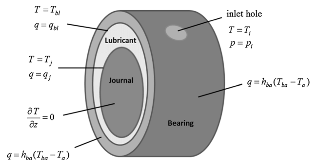
Fig. 3 Thermal boundary conditions
