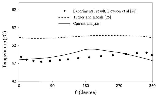
Fig. 8 Comparison of experimental result and current analysis for the circumferential journal surface temperatures for \varepsilon = 0.5 at N = 1,500 rpm
