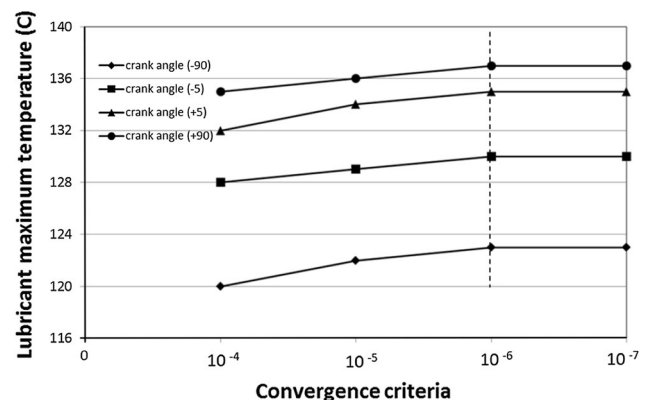
Fig. 18 Lubricant maximum temperature versus different convergence criteria for energy conservation
