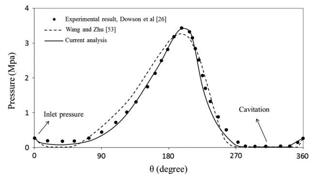
Fig. 6 Comparison of experimental result and current analysis on pressure distribution in the centre plane for \varepsilon = 0.5 at N = 1,500 rpm
