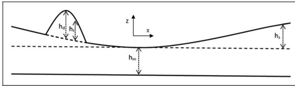
Figure 5. Film shape for rough contact with surface texture.
