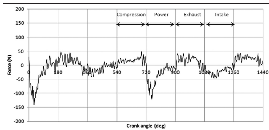
Figure 8. Measured friction under fired engine conditions at an engine speed of 2500 r/min and a torque of 30 N m.
