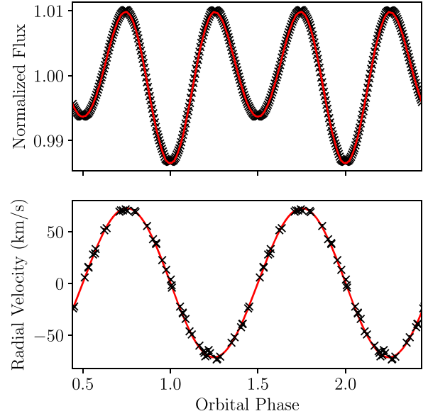
Figure 14. The model PHOEBE2 light curve (top) and RV curve (bottom) overlaid on the observations. In each panel the PHOEBE2 model is in red and the data points are in black. The Doppler boosting term has been removed from the TESS light curve (top panel) before doing the fit.
