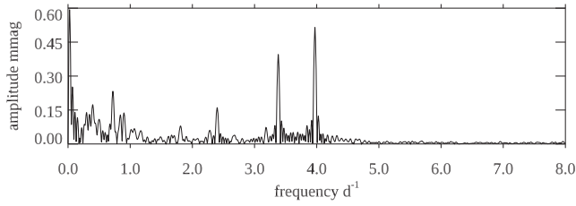
Figure 9. An amplitude spectrum after pre-whitening the orbital harmonic series, showing peaks for at least 3 g modes at 2.398509, 3.380613 and 3.971885 d -1 . The lowest frequency peaks below 1 d -1 are probably instrumental artefacts.
