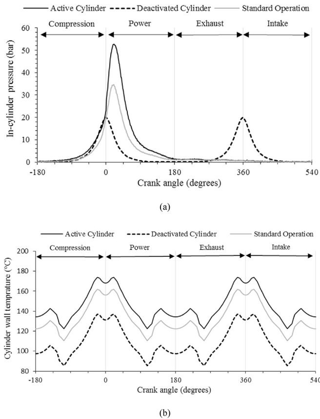
Fig. 4. Measured input data; (a) In-cylinder pressure, (b) Cylinder liner temperature.
