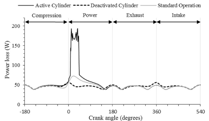
Fig. 9. Big-end bearing power loss.
