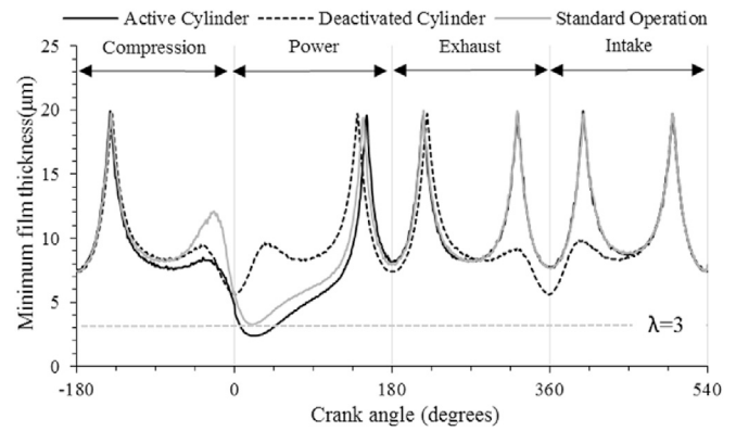
Fig. 8. Big-end bearing minimum film thickness.
