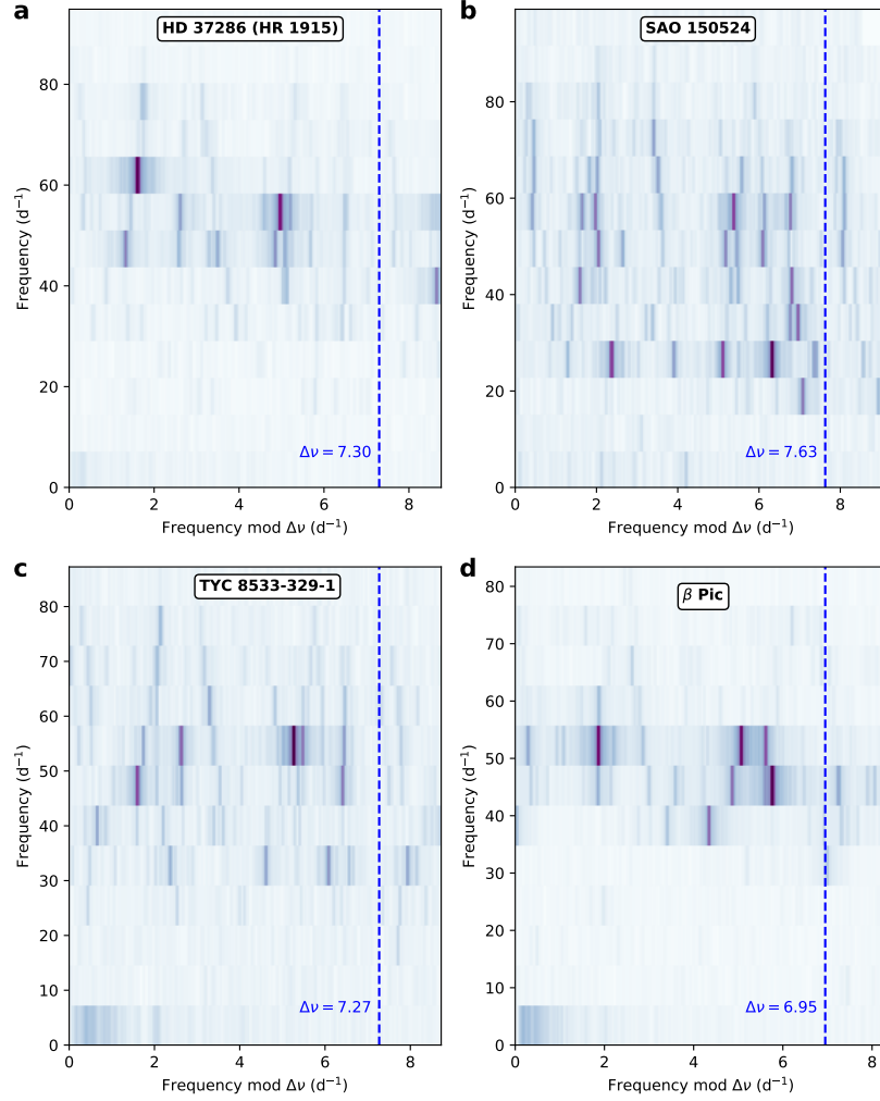
Fig. 4 | Examples of more complicated échelle diagrams of \delta Scuti pulsations. a–d, Diagrams for HD 37286 (=HR 1915; a), SAO 150524 (b), TYC 8533-329-1 (c) and \beta Pic (d). There are sets of ridges at a range of angles, indicating slightly different spacings. An intermediate value of \Delta\nu was chosen for these diagrams (see Methods).
