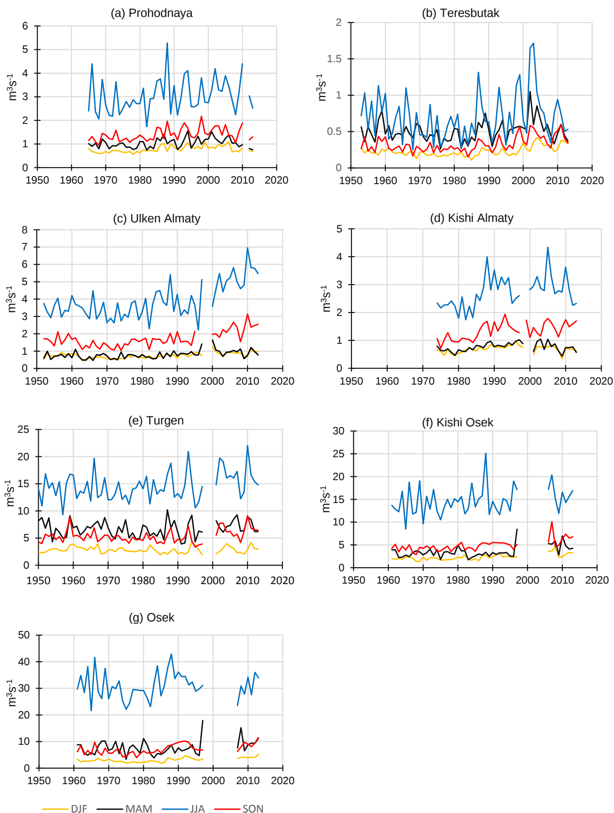
Figure 5. Time series of seasonal mean streamflow ( \text{m}^3 \text{s}^{-1} ). Note that different scales are used for different rivers.
