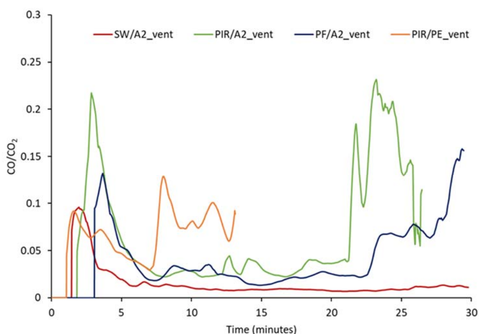
Figure 8 CO/CO 2 ratios
