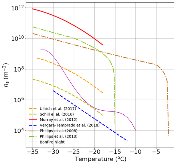
Figure 7. A plot of different BC parameterizations from the literature along with the upper limit to n_s derived in this study of Bonfire Night emissions. The parameterizations from Schill et al. (2016), Ullrich et al. (2017), and Vergara-Temprado et al. (2018) are also upper limits to the activity of BC and were based on laboratory measurements.
