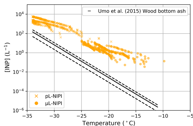
Figure 5. Comparison of a predicted upper limit [INP]_T spectrum for combustion ash compared with measured [INP]_T spectra. The [INP]_T spectrum for ash was based on the measured surface area of mineral dust/ash from the SEM-EDS analysis, assuming that all this material was ash, and the parameterization for wood bottom ash (Umo et al., 2015). The dashed lines represent uncertainties in [INP]_T based upon the uncertainties in the SEM-derived surface area of mineral dust/ash. The [INP]_T measurements and the SEM filters were collected on 4 November 2017.
