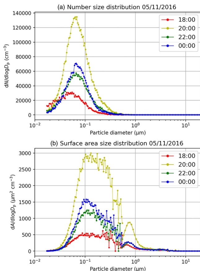
Figure 3. Size distribution of atmospheric aerosol particle populations measured on 5 November 2016 in terms of (a) number concentration and (b) surface area concentration. Size distributions are shown at 2-h increments between 18:00 and 00:00. The x axis is presented in volume equivalent spherical diameter ( D_p ). The electrical mobility data from the SMPS and aerodynamic data from the APS were merged to produce a volume equivalent diameter. This was performed using the method described by Möhler et al. (2008).
