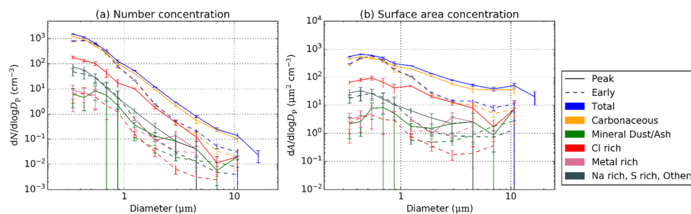
Figure 4. Composition of particles collected on the early (5 November 2017, 16:05–17:25) and peak (5 November 2017, 00:00–00:45) filters in terms of (a) number concentration and (b) surface area. The errors were calculated using Poisson counting statistics. These plots were generated using SEM-EDS analysis.
