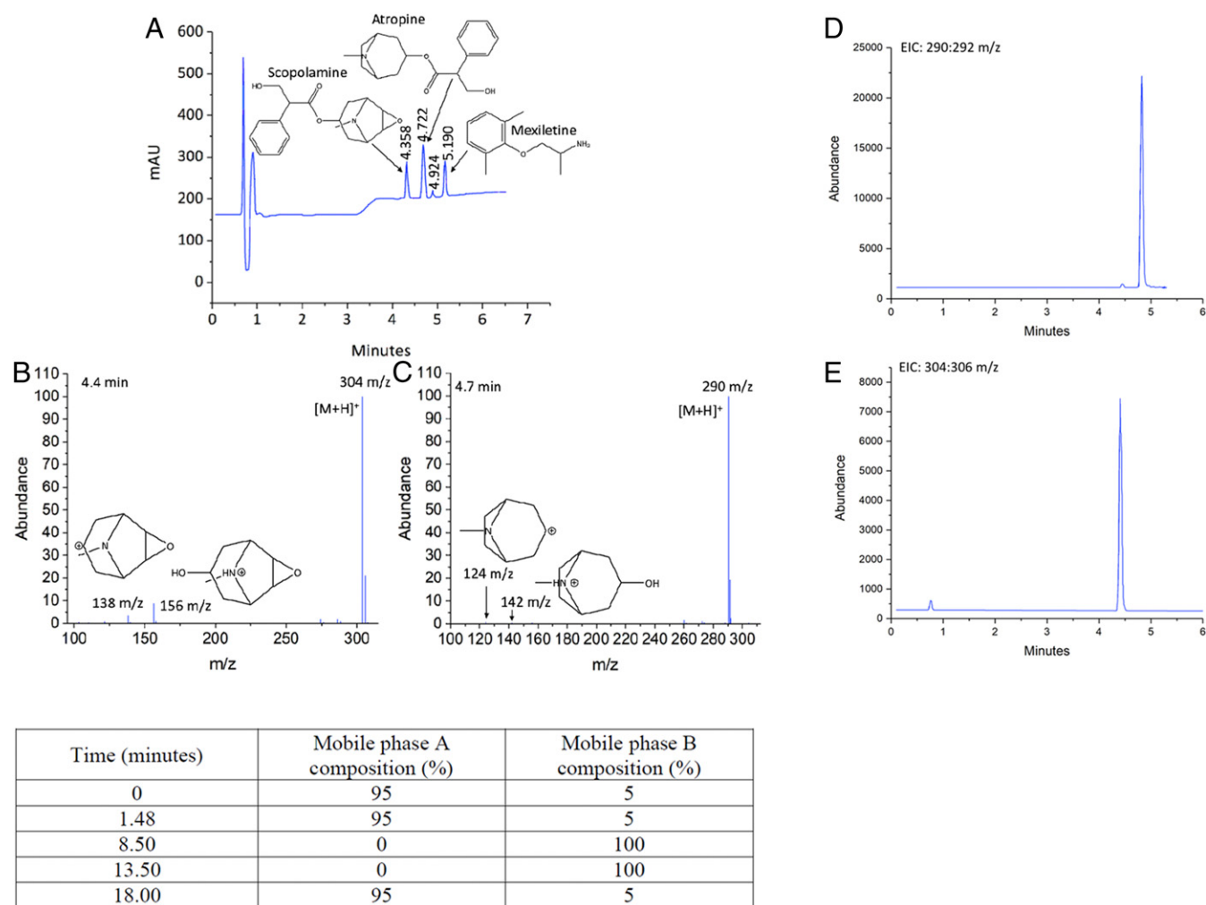
Fig. 4. LC-MS analyses of quids. (A–C) Chromatographic and mass spectrometry data of mixed tropane alkaloid standard. (A) Chromatographic analysis of a mixed standard at concentrations of 0.2 mg·mL -1 for atropine and scopolamine and 0.05 mg·mL -1 for mexiletine recorded at 214 nm. (B) Mass spectra of scopolamine taken across a time range of 4.384 min to 4.477 min, with important fragment peaks highlighted. (C) Mass spectra of atropine taken across a time range of 4.755 min to 4.848 min, with important fragment peaks highlighted. (D and E) Extracted ion chromatograms for Kerr 5832 subsample 4, replicate 2. (D) EIC of atropine over 290 to 292 m/z range. (E) EIC of scopolamine over 304 to 306 m/z range. (Bottom) Table of LC-MS gradient flow profile details, where mobile phase A was 0.1%vol/vol formic acid water and mobile phase B was 0.1%vol/vol formic acid acetonitrile.
