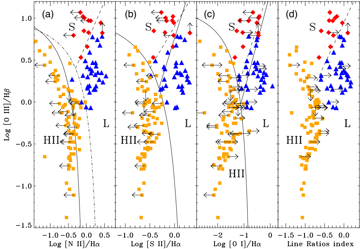
Figure 1. Diagnostic diagrams based on optical spectra (named BPT, Baldwin, Phillips & Terlevich 1981): \log([O\text{ III}]/H\beta) versus (a) \log([N\text{ II}]/H\alpha) , (b) \log([S\text{ II}]/H\alpha) , (c) versus \log([O\text{ I}]/H\alpha) , and (d) line ratios index (the averaged line ratios, see the definition in Paper I). The data-points represent the 122 galaxies with emission line data taken from Ho et al. (1997) (the remaining 55 sources were classified based on data from the recent literature; see Table 1). In the first three panels, the solid lines separating H II galaxies, LINER, and Seyferts are taken from Kewley et al. (2006). The dashed lines between Seyferts and LINERs in the four panels separate the two classes according to the scheme introduced by Buttiglione et al. (2010). In panel (a), the sources between the solid and the dot-dashed lines were classified as transition galaxies by Ho et al. (1997), which we re-classify as LINER or H II galaxies based on the other diagrams ('b' and 'c'). We mark LINERs as blue triangles, Seyferts as red diamonds, and H II galaxies as orange squares. Several galaxies have different classifications with respect to those from Ho et al. (1997) because of the updated diagnostic diagrams (see Table 1).
