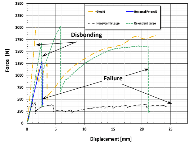
Fig 10 Loading force in Newtons against displacement for (a) HL, RL, HP and G and (b) HS, RS and P cores.
