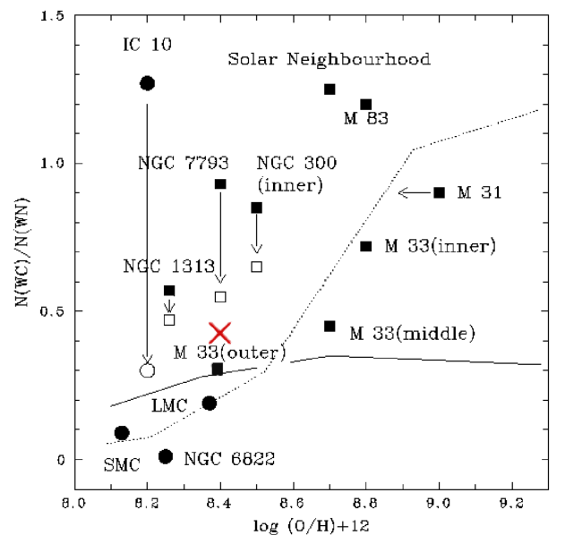
Figure 6. Adapted from Bibby & Crowther (2010; their fig. 13a) showing the WC/WN ratio in a number of galaxies at different metallicities. The observed ratios are plotted as solid points and the ratio corrected for WC bias and detection limits are the open points. The WC/WN ratio for NGC 7793 is additionally corrected for spatial resolution and line dilution using this work and is indicated by the red X. The result for NGC 7793 is more in line with evolutionary predictions from Eldridge & Vink (2006) (dotted line) and Meynet & Maeder (2005) (solid line).
