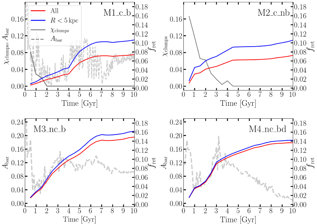
Figure 3. The time evolution of the retrograde mass fraction, f_{\text{ret}} = M_{\text{ret}}(t)/M_*(10 \text{ Gyr}) , in the four models, where M_{\text{ret}}(t) and M_*(10 \text{ Gyr}) are the total mass of retrograde stars at time t and the total stellar mass at the end of the models, respectively. The red lines show f_{\text{ret}} for all stars, while the blue lines reflect f_{\text{ret}} inside 5 kpc, with M_*(10 \text{ Gyr}) being the total stellar mass also inside this region. The solid and dashed grey lines reflect the clumpy mass fraction and the bar amplitude, respectively. In both cases the scales for the grey lines are presented on the left hand axis.
