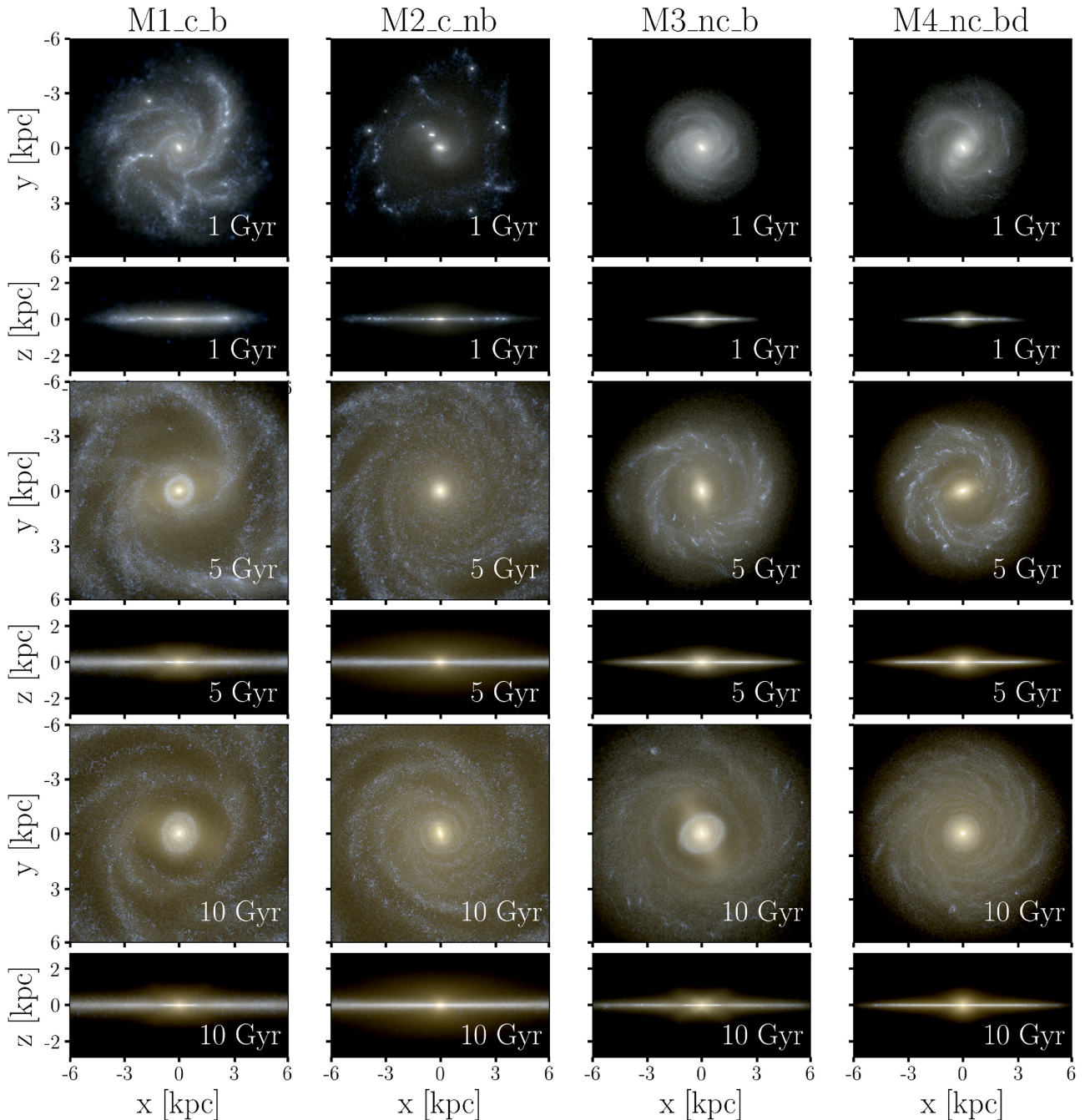
Figure 1. Synthetic RGB images produced with PYNBODY of the stellar discs of the models. We show the models both face-on and side-on at 1 Gyr (top two rows), then at 5 Gyr (next two rows), and at 10 Gyr (bottom two rows). These images highlight the different evolutionary paths the models take. The clumpy nature of M1_c_b and M2_c_nb early in their evolution may also be contrasted with M3_nc_b and M4_nc_bd, which do not go through a clumpy episode.
