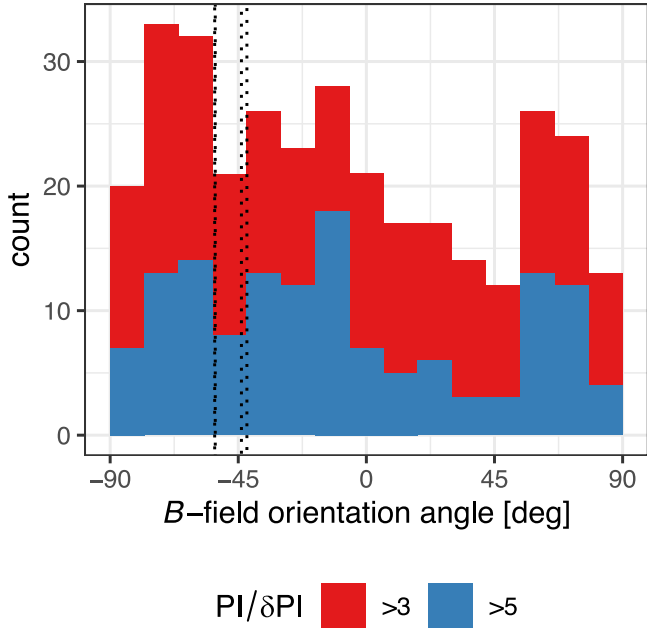
Figure 5. Histogram of the position angles for the B -field orientations ( \psi + 90^\circ ) shown in Figure 4. The typical estimation error of \psi(1\sigma) is 4^\circ for PI/\delta PI > 5 and 5^\circ for PI/\delta PI > 3 . So we set the bin size of the histogram as 12^\circ . Dotted lines indicate the B -field orientation observed with Planck within the JCMT field of view (see the yellow line segments in Figure 4). The distribution of position angles is estimated as -46^\circ \pm 58^\circ for the B -field orientation observed by JCMT and -48^\circ \pm 6^\circ for that by Planck.
