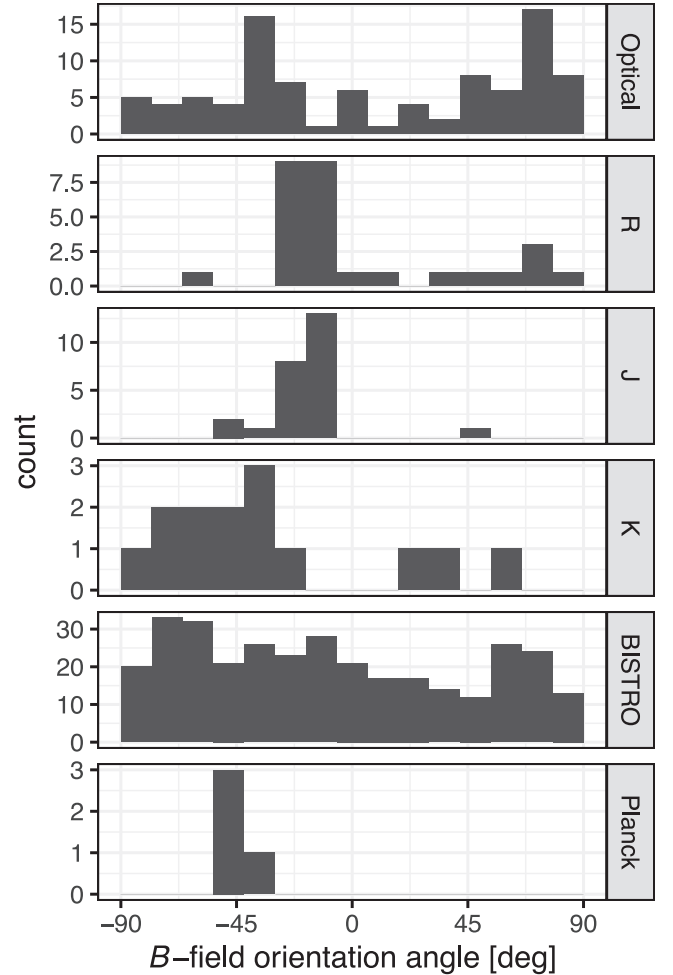
Figure 10. Histograms of the position angles for the B -field orientations observed by optical and near-infrared polarimetry. Optical data (762.5 nm) are from Goodman et al. (1990). R -band data are from Alves et al. (2011). J -band data are from Tamura et al. (1988). Submillimeter data taken by BISTRO and Planck, rotated by 90^\circ , are shown for comparison. Note that the spatial coverages are different for individual observations, especially R -band and J -band data by Alves et al. (2011), which cover only a small area south of the IRAS 4A and IRAS 4B (see text).
