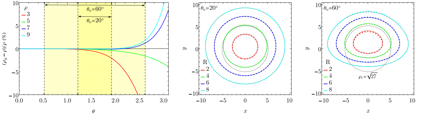
Figure 11. Testing the accuracy of the Beloborodov approximation. The left panel shows fractional error in \rho = \sqrt{x^2 + y^2} as a function of \psi for \rho = 3, 5, 7 , and 9 . Yellow ranges denote values of \psi relevant for observer inclinations \theta_o = 20^\circ and 60^\circ . The center and right panels show the image coordinates for rings with emission radius R = 2 (red), 4 (green), 6 (blue), and 8 (cyan) viewed at inclinations of 20^\circ and 60^\circ , respectively. For each ring, the solid line shows the exact calculation, while the dotted line shows the Beloborodov approximation (see Equation (C4)). The black dotted line shows the critical curve, \rho = \rho_c \equiv \sqrt{27} .
