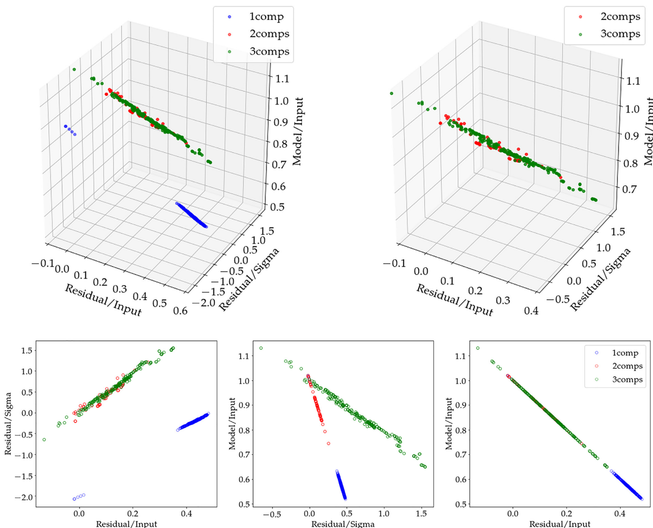
Figure A1. GALFITM models created for NGC 3115 using one, two, and three components, with different combinations of orders that define how each parameter can vary with the wavelength. Models are evaluated according to the statistics: Residual/Input (how the residual compares with the input image: the smallest the better), Residual/Sigma (how the residual compares to the error of the input image, the smallest the better), and Model/Input (how well the model is mimicking the input image: the closest to one the better). The bottom line shows the 2D projection of each pair of axes of the 3D plot for the models with one, two, and three components.
