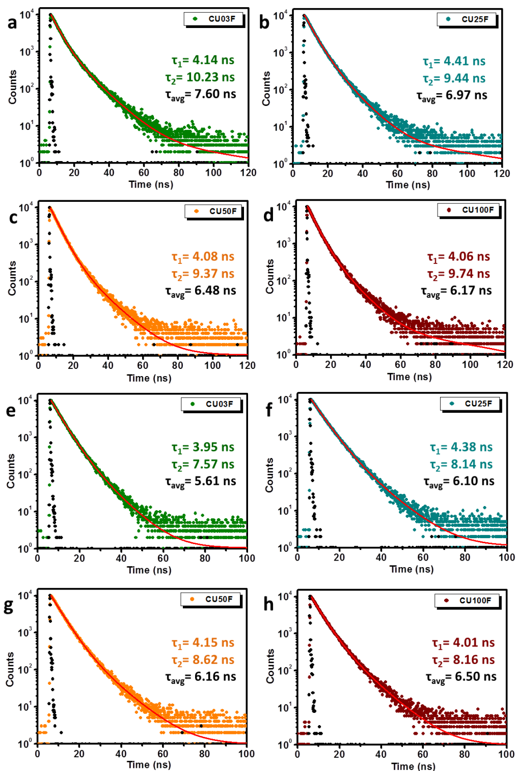
Figure S15. Fluorescence lifetime decays of 0.1 mg /ml aqueous dispersions of CU03F, CU25F, CU50F and CU100F at \lambda_{ex}= 375 nm (a-d) and \lambda_{ex}= 450 nm (e-h). The points represent the experimental data and the lines correspond to cumulative fitted curves.
