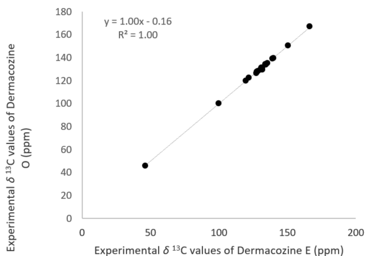
Figure 8. Correlation between the experimental ^{13}\text{C} -NMR chemical shift values (ppm) of dermacozine O (2) and the experimental ^{13}\text{C} -NMR chemical shift values (ppm) of dermacozine E (8).
