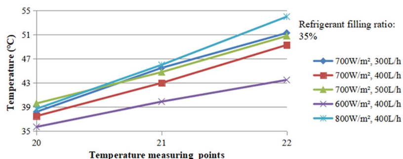
Figure 11. Temperature variation of the MCFLHP under the refrigerant filling ratio of 35% condition (P20–P22 in the No. 33 heat pipe).
