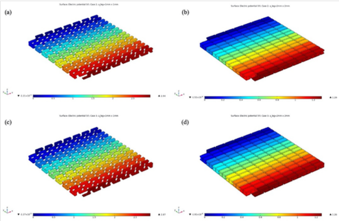
Electric potential plots for leg area of (a, c) 1 mm 2 and (c, d) 4 mm 2 .
