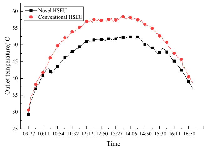
Fig. 21. The variation of the outlet temperature of the solar thermal array
