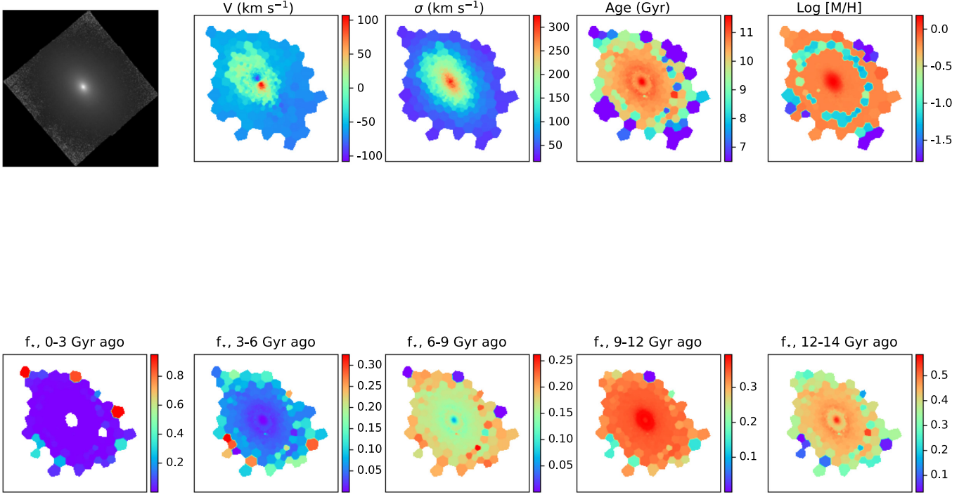
Figure B3. IC 1459. Top left-hand panel shows the collapsed MUSE cube. Other top row panels show stellar parameters of velocity, velocity dispersion, age, and metallicity. Lower panels show stars selected by age. Colour shows the fraction of stars in a bin that are of a specific age.
