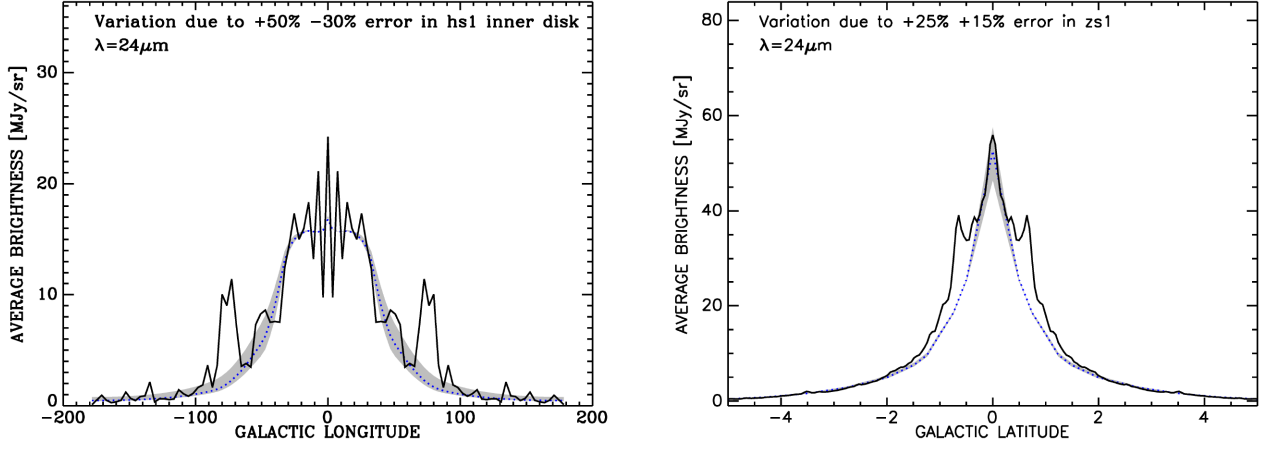
Figure C3. Left-hand panel: Variation in the average longitude model profiles (shaded area) of surface brightness at 24\ \mu\text{m} due to +50 per cent – 30 per cent variation in the h_s^{\text{in-tdisc}} and a change in the \text{SFR}^{\text{in-tdisc}} \times F^{\text{in-tdisc}} parameter, such that the centre region of the 24\ \mu\text{m} longitude profile is fitted. Right-hand panel: Variation in the average latitude model profiles (shaded area) of surface brightness at 24\ \mu\text{m} due to +25 per cent – 15 per cent variation in the z_s^{\text{in-tdisc}} and a change in the \text{SFR}^{\text{in-tdisc}} \times F^{\text{in-tdisc}} parameter, such that the centre region of the 24\ \mu\text{m} longitude profile is fitted. The corresponding observed profiles are plotted with a solid line.
