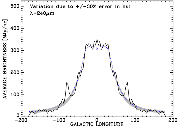
Figure C4. Variation in the average longitude model profiles (shaded area) of surface brightness at 240\ \mu\text{m} due to 30 per cent variation in the h_s^{\text{tdisc}} and a change in the \text{SFR}^{\text{tdisc}} \times (1 - F)^{\text{tdisc}} parameter, such that the centre region of the 240\ \mu\text{m} longitude profile is fitted.
