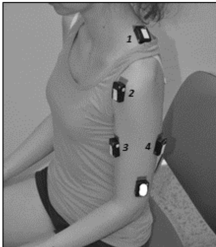
Figure 2. Illustrative sensors placement. In white-coloured is arm IMU sensor for spatiotemporal data. Sensors (1-4) are for electromyographic data, where 1 is Upper Trapezius, 2 Anterior Deltoid, 3 Biceps Brachii, 4 Triceps Brachii
