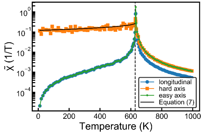
FIG. 4. Susceptibilities computed using a 30\text{ nm}^3 mesh and uniaxial anisotropy along the x axis, with K = 5 \times 10^{-23} J. The variance in Equation (6) is obtained from a set of 50,000 atomistic ensembles at each temperature. For the longitudinal susceptibility \alpha = l , for the easy axis susceptibility \alpha = x , and for the hard axis susceptibility (transverse susceptibility) we average the results for \alpha = y and \alpha = z . The latter is compared to the transverse susceptibility obtained from Equation (7), shown as a solid line, with m(T) and K_u(T) computed separately for the same mesh size. The vertical dashed line indicates the Curie temperature of 628.0 K.
