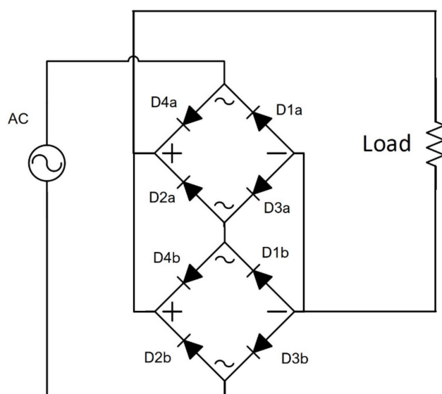
Figure 4. Multicell bridge ISOP circuit.
