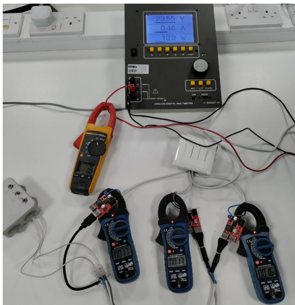
Figure 9. Experimental set-up of load sharing between parallel buck cells.
