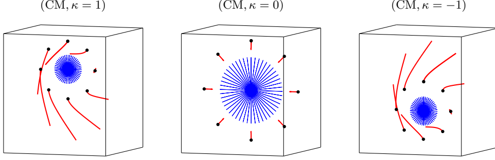
Figure 2: Three-dimensional spacecurves for particles subject to an incident (CM,1) laser pulse (left), (CM,0) laser pulse (centre) and (CM,-1) laser pulse (right) with parameters \{\Lambda = 600, \Psi_1 = 1, \Psi_2 = 1000, \Phi = 0.001, \Xi = 1\} . Each particle has initial velocity \{\dot{R}(0) = 0, \dot{\theta}(0) = 0, \dot{Z}(0) = \frac{1}{200}\} . The shaded circular disc region indicates the initial spot size ( R = 10000 for (CM, \pm 1 ) laser pulses and R = 20000 for a (CM, 0) laser pulse) relative to the black markers on the spacecurves that denote the initial positions of the charged test particles.
