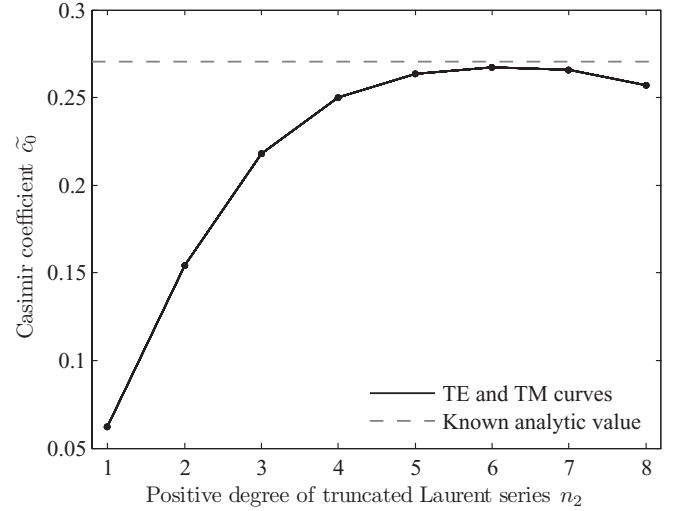
FIG. 1. For data based on (3), the algorithm determines \mathcal{N} = -4 and a collection of [x, y] points [\hat{n}_2, \hat{c}_0(\mathcal{N}, \hat{n}_2, n_2)] with 1 \leq n_2 \leq 8 . The eight curves obtained by joining these points are indistinguishable in this figure and the average of \hat{c}_0(\mathcal{N}, \hat{n}_2, n_2) at their turning points yields a Casimir coefficient c_0(\mathcal{N}) = 0.27281 . The horizontal dotted line indicates the value of the Casimir coefficient that determines the observed Casimir attractive pressure between perfectly conducting plates separated by the vacuum.
