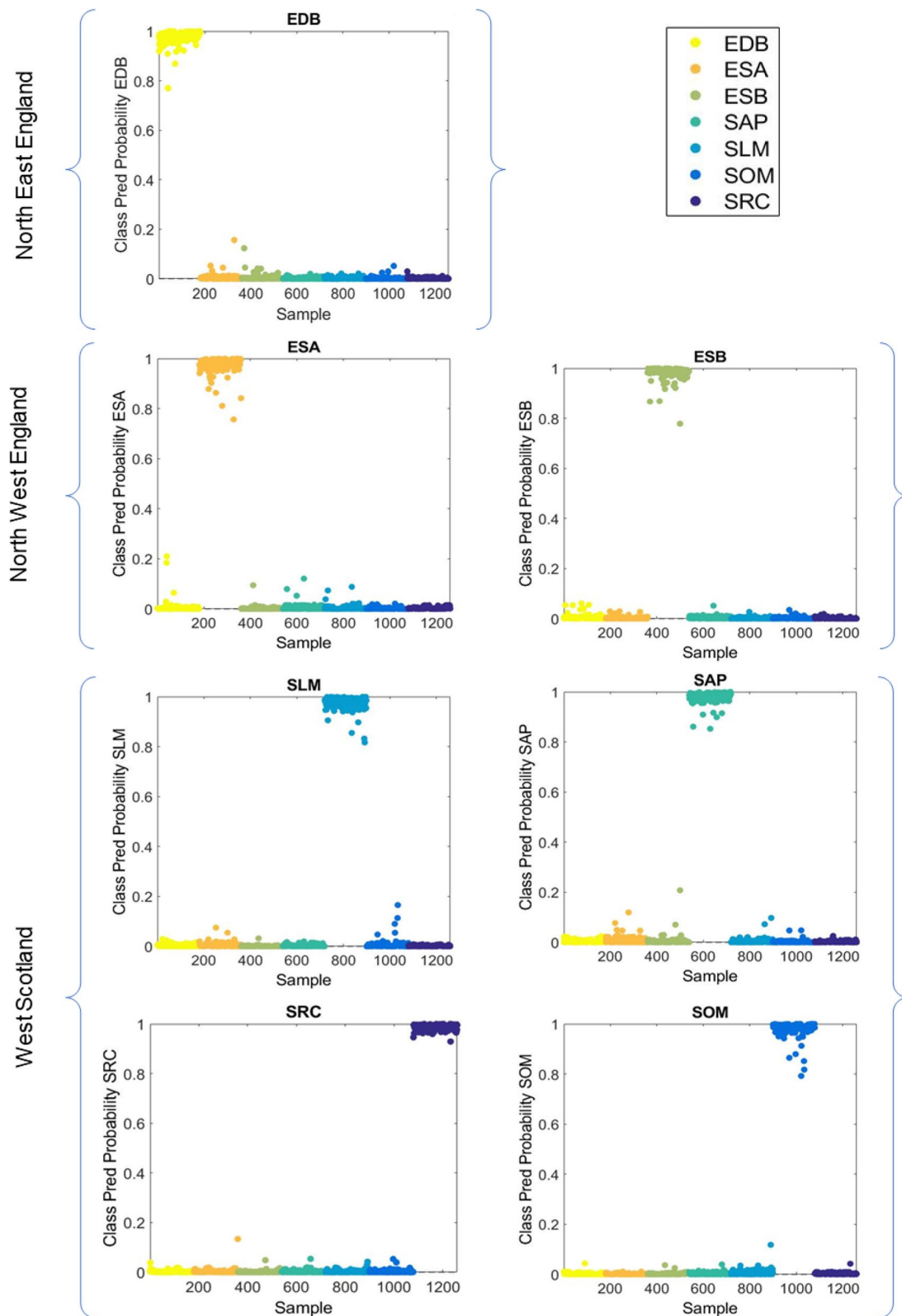
Fig. 4 SVM class predicted probability for the IR spectral dataset according to different sites where knotweed samples were collected (Scotland: SRC, SOM, SLM, SAP; North West England: ESA, ESB; North East England: EDB). The clear separation indicates that the knotweed samples can be differentiated by the site at which they were collected
