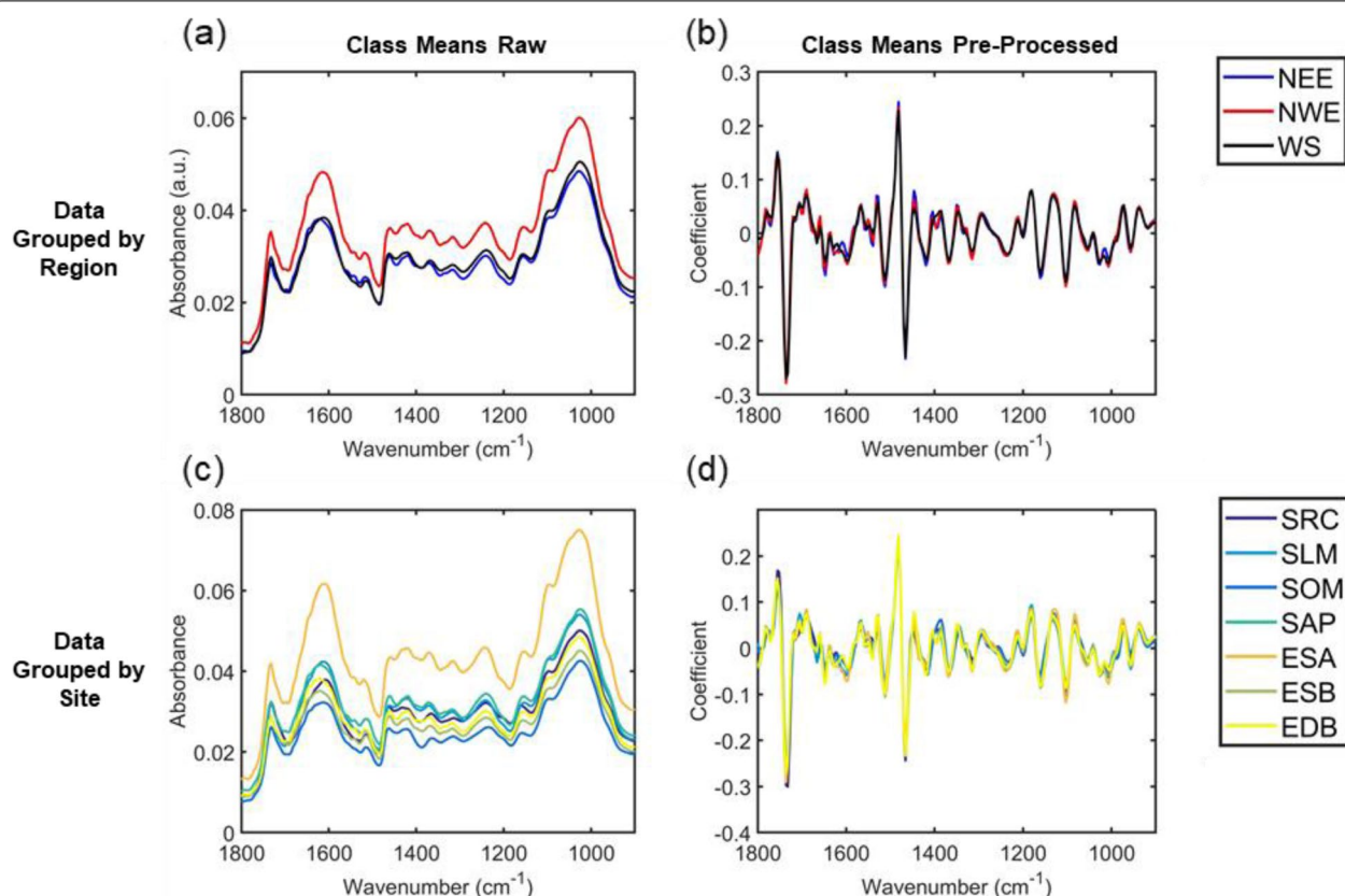
Fig. 1 (a) Class means raw and (b) class means pre-processed (SG smoothed and vector normalised) IR spectra in the fingerprint region (1800–900 \text{cm}^{-1} ) grouped by the different regions where knotweed samples were collected (NEE: North East England, NWE: North West England, WS: West Scotland); (c) class means raw and (d) class means pre-processed (SG smoothed and vector normalised) spectra in the fingerprint region (1800–900 \text{cm}^{-1} ) grouped by the different sites where knotweed samples were collected (Scotland: SRC, SOM, SLM, SAP; North West England: ESA, ESB; North East England: EDB)
