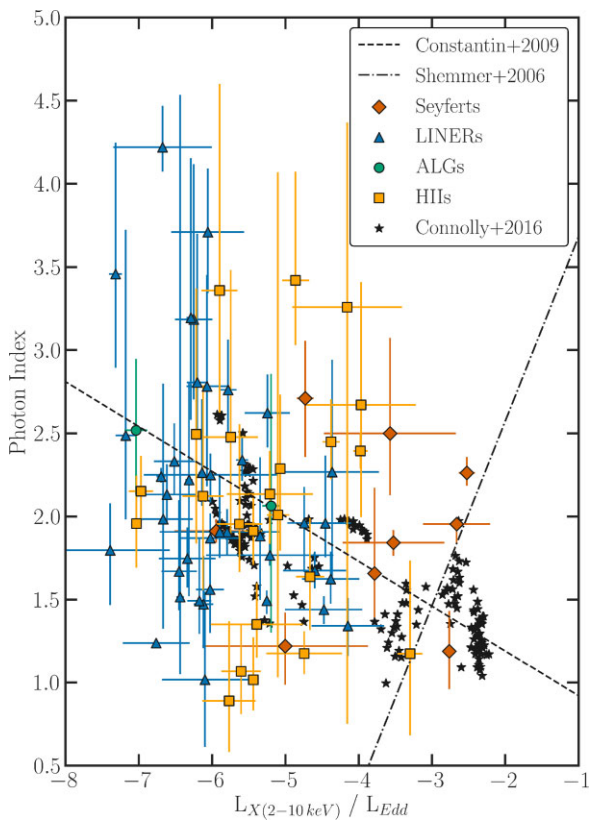
Figure 14. Photon index of the entire sample where reliable photon indices were extracted from the spectra and the source luminosity is >10^{39} \text{ erg s}^{-1} plotted against the tracer of the accretion rate, defined by the ratio between L_{X\text{-ray}} (2–10 keV) and L_{\text{Edd}} , split by different AGN types. We also plot the results from the study by Connolly et al. (2016), which includes a sample of 24 Palomar galaxies, but we include averaged values of the data points included in that study. The lines correspond to the fits from Shemmer et al. (2006) for higher Eddington rate radio-quiet AGN and Constantin et al. (2009) for LLAGN.
