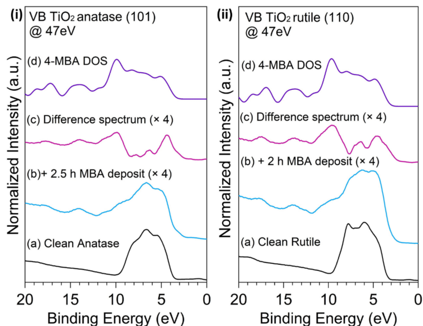
Figure 6. Valence band spectra recorded at 47 eV from the (i) clean anatase, and (ii) clean rutile \text{TiO}_2 surfaces following the adsorption of the 4-MBA molecule.
