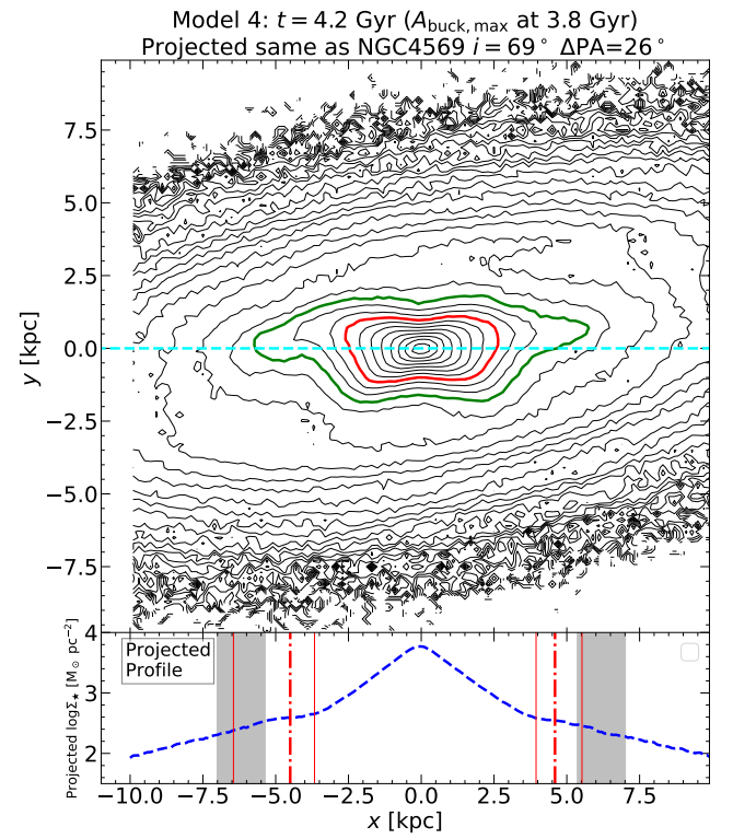
Figure 21. Upper panel: \log \Sigma_{\star} density contours in the projected ( x , y )-plane for model 4 during its buckling at time t = 4.2 Gyr, 0.4 Gyr after maximum A_{\text{buck}} . The model has been rotated to match the inclination and bar relative position angle of NGC 4569. The dashed cyan line represents the projected bar’s major axis, which has been rotated to lie along the projected x -axis. A sample trapezoidal inner isodensity contour is shown in red, and in green is a contour with spurs offset on the same side of the major axis; these are the observational signatures of a buckling bar. Lower panel: \log \Sigma_{\star} along the projected bar major axis, x (projected |y| \leq 1 kpc). The grey area represents the projected bar radius, the vertical dot-dashed lines represent the clavicle centres as identified by the SRA, and the thin vertical red lines mark the boundaries of the shoulders.
