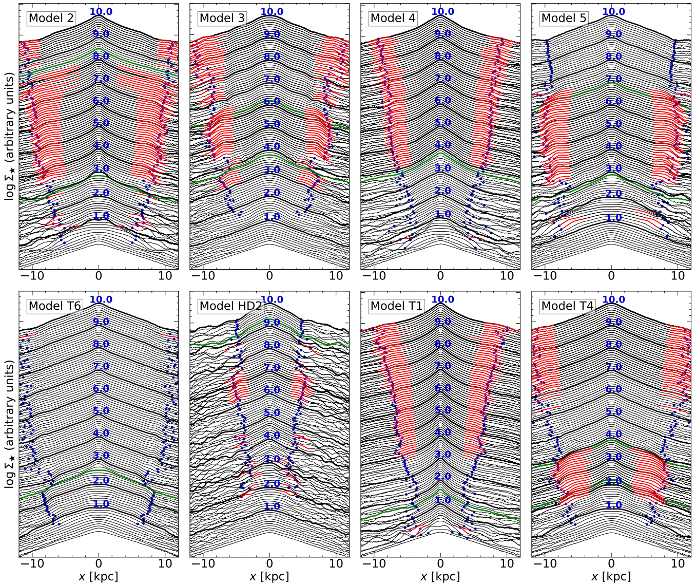
Figure 7. Evolution of the logarithmic surface density profile in the major axis cut for group B models (except model 2S which is shown in Fig. 8). Time advances along the vertical axis. Every 1 Gyr, the profile is highlighted in bold and the time in Gyr indicated above the maximum density. The blue dots represent the bar radius. If the SRA recognises a shoulder, its extent (inner to outer edge) is shown in red. The times of major buckling episode peaks are shown in green. Shoulders, if present, usually appear after first buckling.
