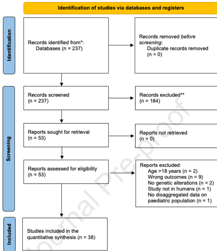
Figure 1. PRISMA diagram
