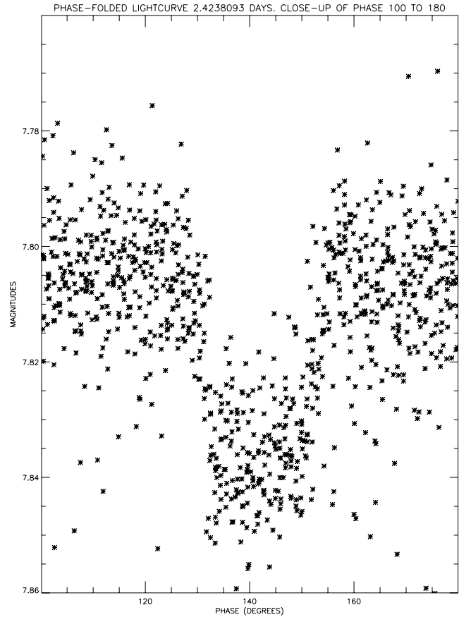
Figure 21. Close-up of the transit of HD 213597, phase-folded on a period of 2.4238 d. This light curve was constructed using the latest data available, including updated flat-fields as well as data from the STEREO /HI-1B.
