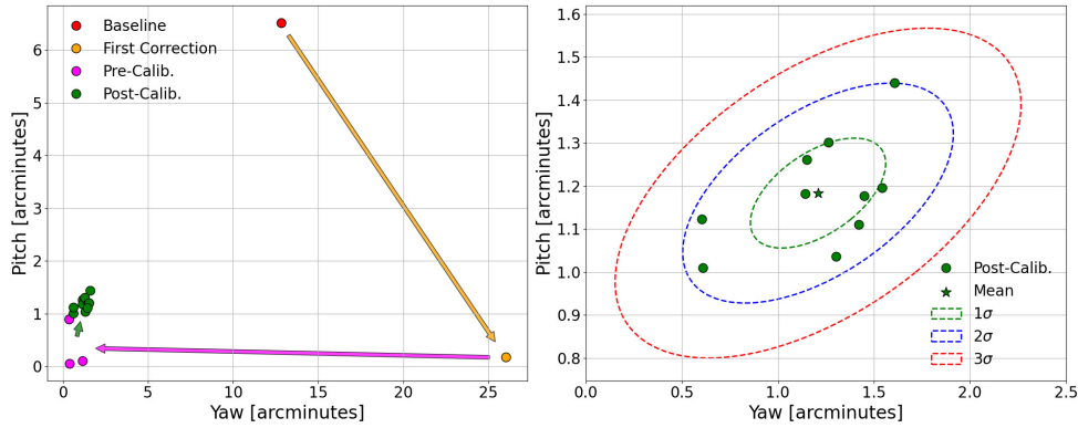
Fig. 17. The TMA-SOA alignment. Each point is a theodolite measurement of the TMA and SOA reference mirror offset. The left panel shows the evolution from the initial mounting of the SOA to the optical bench, to when the system was aligned. The right panel is rescaled to show the cluster of TMA to SOA alignment measurements taken post-calibration. The 1, 2, and 3 \sigma confidence ellipses are plotted for the post-calibration measurements.
