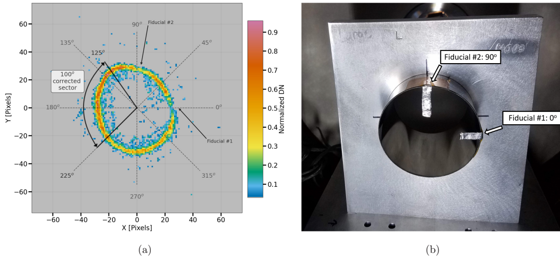
Fig. 6. Left: An X-ray image produced by Spectrometer Mirror 1 (SM1) with the detector placed 6 mm inside of the mirror's focal plane. The sector bound by azimuth angles \theta = 125^\circ to \theta = 225^\circ had figure errors corrected via the deterministic polishing process. Right: SM1 in a test mount, looking at the entrance aperture from the direction of the source. Two fiducials were placed at the 0^\circ and 90^\circ locations that are meant to block X-rays, creating two shadows in the image that are used to register the clocking of the exit pupil.
