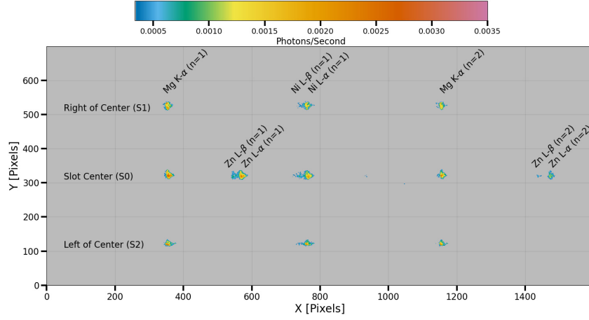
Fig. 18. The composite X-ray image containing all of the data collected from the fully integrated calibration tests. First- and second-order spectra were detected for the Mg-K \alpha and Zn-L \alpha, \beta lines. The first-order Ni-L \alpha, \beta line is detected near the center of the image, with the second-order line falling just off to the right side of the detector.
