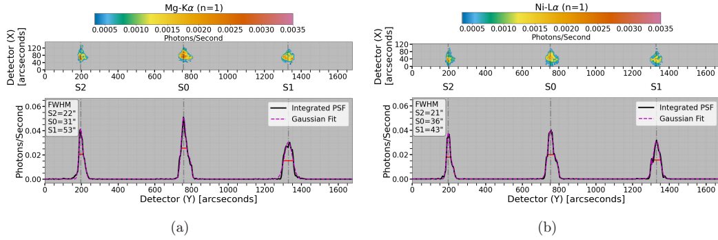
Fig. 19. Images of the focused spots and PSF profiles for the Mg-K \alpha ( n = 1 ) (left panel) and Ni-L \alpha ( n = 1 ) (right panel). The PSF profiles are the result of integrating over the spots in the dispersion axis (Detector X -axis). A sum of two 1D Gaussian functions were fit to each of the three spot profiles and are over-plotted onto the profiles as the fuchsia dashed line. The vertical dashed-dot gray lines indicate the mean of Gaussian fit to the core, and the horizontal red lines denote the FWHM.
