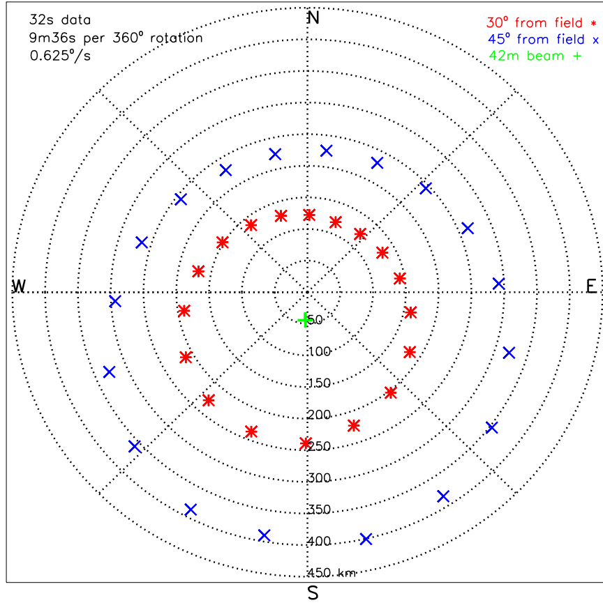
Figure 1: Scan pattern - distance from 32m antennae (km) at height 300 km. (Green: position of 42m field-aligned beam; red: data-points at 30^\circ from field; blue: data-points at 45^\circ from field.) The patterns are not symmetrical with respect to the 42m beam because the section is horizontal, not orthogonal to that beam.
