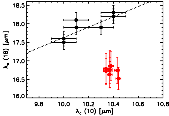
Figure 5. The central wavelengths of the 9.7 \mu\text{m} and 18 \mu\text{m} features in RS Oph (red circles from Table 1) and symbiotic stars (black circles) from Angeloni et al. (2007). The dotted line is an empirical relation for symbiotic stars from Angeloni et al.
