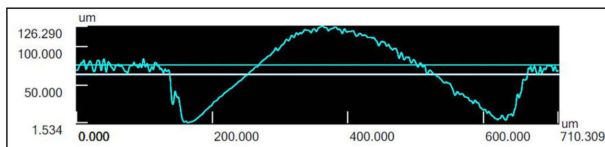
Figure 7. Measured lip seal profile.
