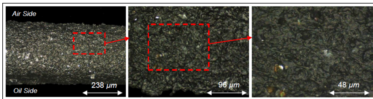
Figure 8. Topographical surface features of the lip seal under 20\times , 50\times and 100\times optical magnifications.
