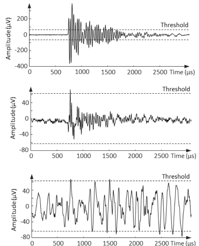
Fig. 3. Example AE waveforms: strong transient wave (top), weak transient wave (middle), and weak continuous wave (bottom)
