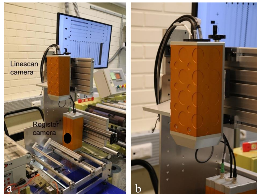
Figure 2. (a) Line scan camera and register camera installed on a reeling machine. (b) Close-up image of the line scan camera.
