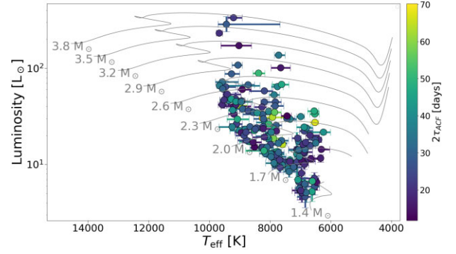
Figure 16. HR diagram with symbols correlated with the spike lifetime as calculated in Section 2.6. The source for luminosity and T_{eff} values is described in Section 2.3. Warsaw–New Jersey evolutionary tracks ( Z = 0.012 , Asplund et al. 2004) are displayed in the background for guidance only.
