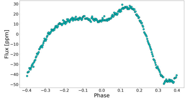
Figure 25. Phase-folded light curve computed with the full Kepler time series – KIC 3440710 (group A – see Section 4.3.2); average bin size \sim 0.003 in phase; folded on period \sim 0.8 d; which corresponds to the frequency of the main spike \sim 1.25 d ^{-1} .
