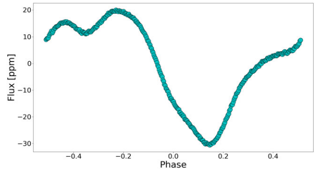
Figure 21. Phase-folded light curve computed with the band-passed filtered time series of KIC 4661914 (group C – see Section 4.3.2); average bin size \sim 0.003 in phase folded on period \sim 1.024 \text{ d} which corresponds to the frequency of the main spike \sim 0.977 \text{ d}^{-1} .
