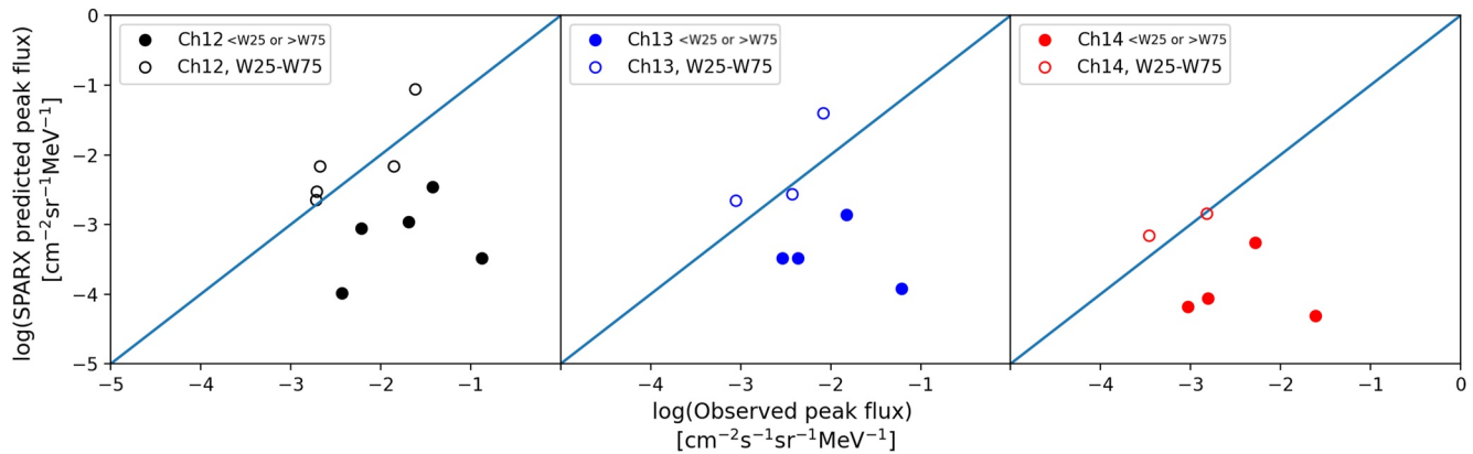
Figure 3. The observed and SPARX–H predicted logarithm of the peak fluxes for the historic test solar energetic particle events over the three high energy channels. Unfilled circles show events with associated flare longitudes between W25 and W75. The blue line is the 1:1 line.
