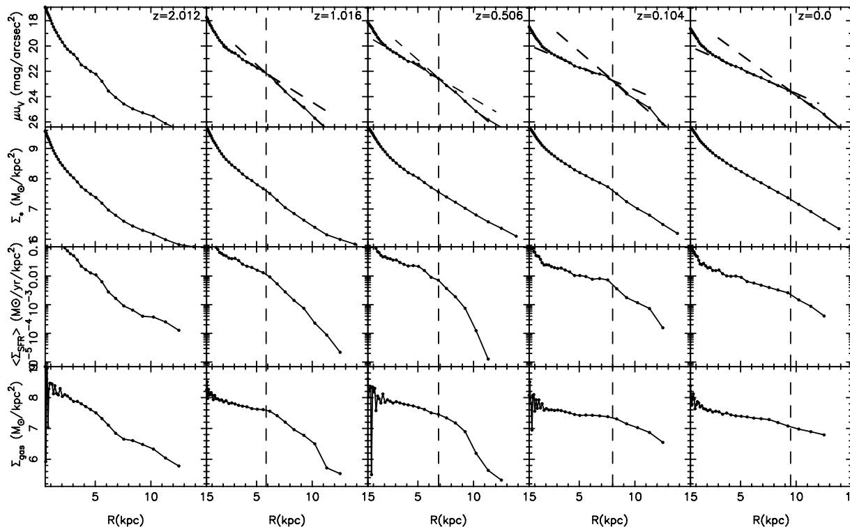
Figure 4. Evolution with redshift – as indicated in the inset to each panel – of the V -band surface brightness profile (first row), total stellar surface density profile (second row), SFR surface density profile (third row) and gas surface density profile (fourth row), all on logarithmic scales. The profiles were derived using all stars with r < 15 kpc and |z| < 3 kpc. Dashed lines represent fits to the inner and outer exponentials in the V -band surface brightness profile. The break radii correspond to the intersection point of these two exponentials, and are noted by the vertical dashed lines in each panel.
