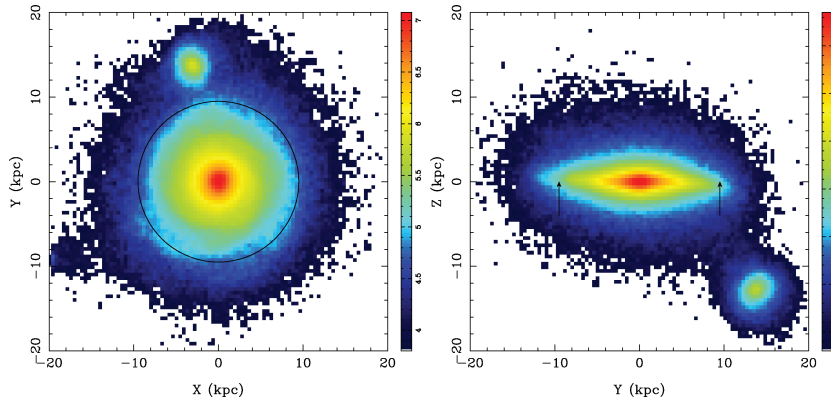
Figure 3. Stellar density projections of the disc (left-hand panel: face-on; right-hand panel: edge-on). A 40 \times 40 kpc region is shown in both the panels. The circle in the left-hand panel and the arrows in the right-hand panel indicate the position of the break radius (see Section 4).
