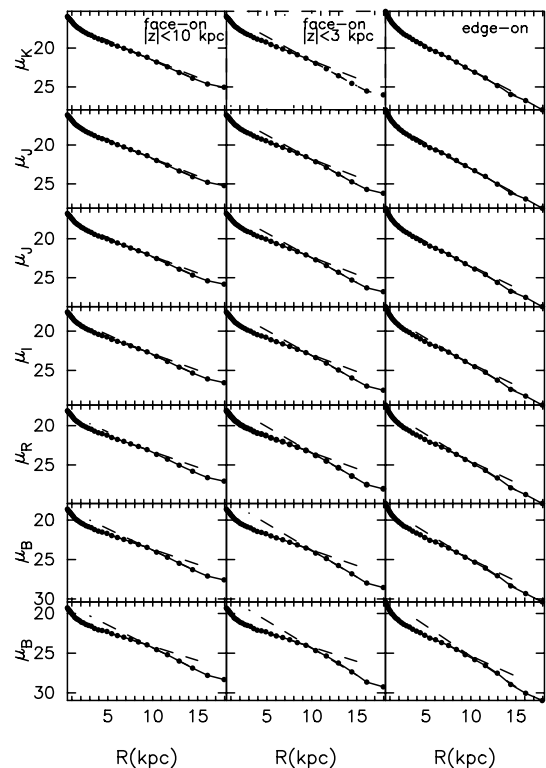
Figure A1. Surface brightness profiles in different bands calculated in face-on (azimuthally averaged) and edge-on configurations. For the face-on projection, we have integrated between different distances from the disc mid-plane, as indicated in the inset.
