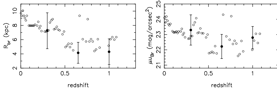
Figure 11. Predicted evolution with redshift of R_{\text{br}} and \mu_{\text{br}} (open circles) compared to the observed values from Azzollini et al. (2008) (filled circles with error bars). The error bars show the rms dispersion of the measured values for galaxies in a given redshift bin and mass bin.
