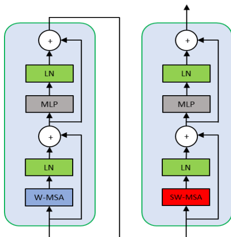
Figure 1: Two successive SwinV2 Transformer Blocks [13]. The residual post normalization configuration ensures layer normalization is conducted after attention layers and MLP layers.
