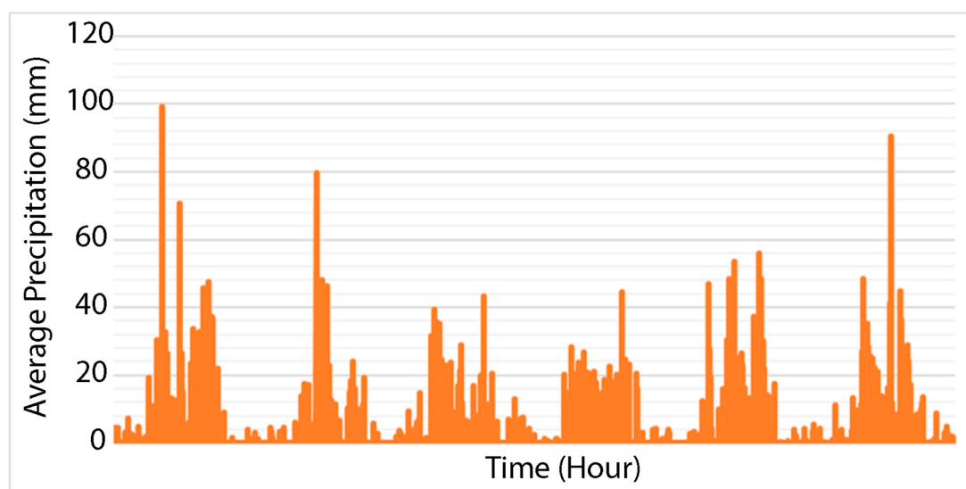
Figure 4. Hourly precipitation, 2010–2015.
