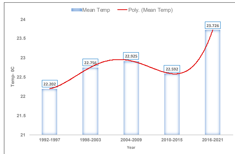
Figure 10. Trend analysis: temperatures (1992–2021).
