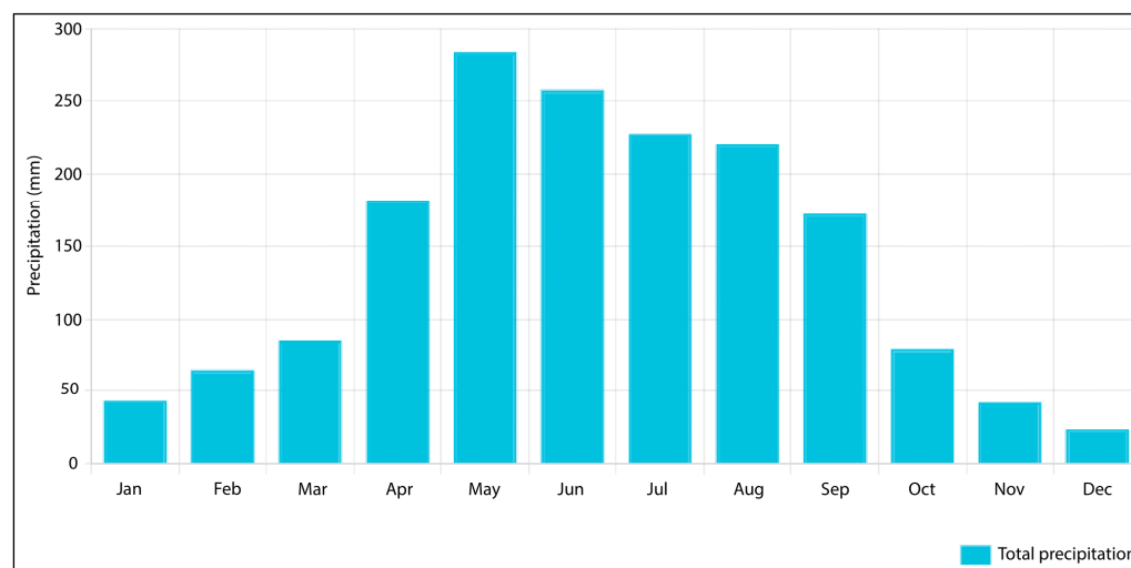
Figure 2. Monthly precipitation, 1961–1990.
