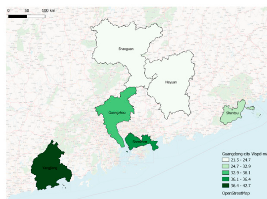
Peak value of windspeed, 1991–2022.
