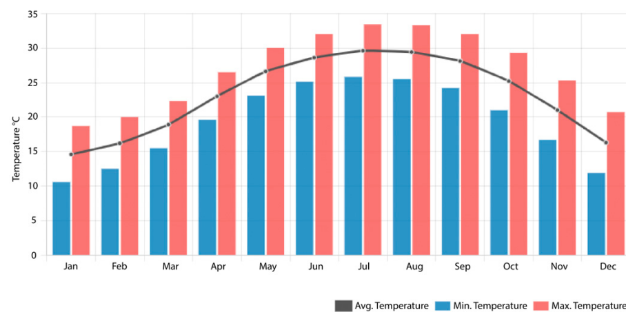
Figure 5. Average monthly temperature, 1961–1990.
