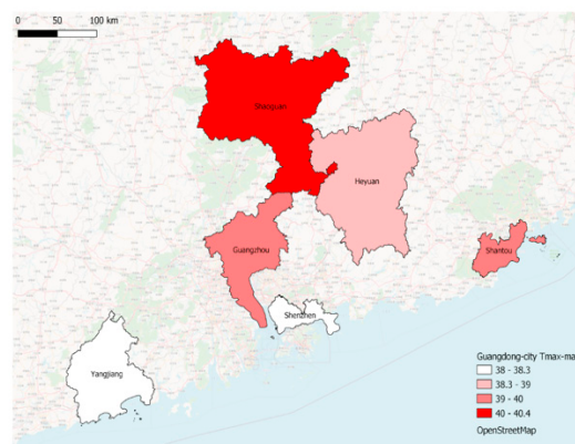
Peak value of temperature, 1991–2022.
