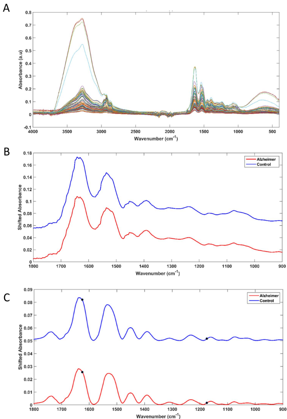
Figure 2. A. Raw spectra after analysis of buccal cells with ATR-FTIR. B. Mean spectra of Alzheimer's disease patients and controls in the fingerprint region ( 1800\text{--}900\text{ cm}^{-1} ). C. Mean pre-processed spectra of Alzheimer's disease patients and controls along with the most important wavenumbers for classification selected by SPA-QDA ( 1628\text{ cm}^{-1} , 1181\text{ cm}^{-1} ).
