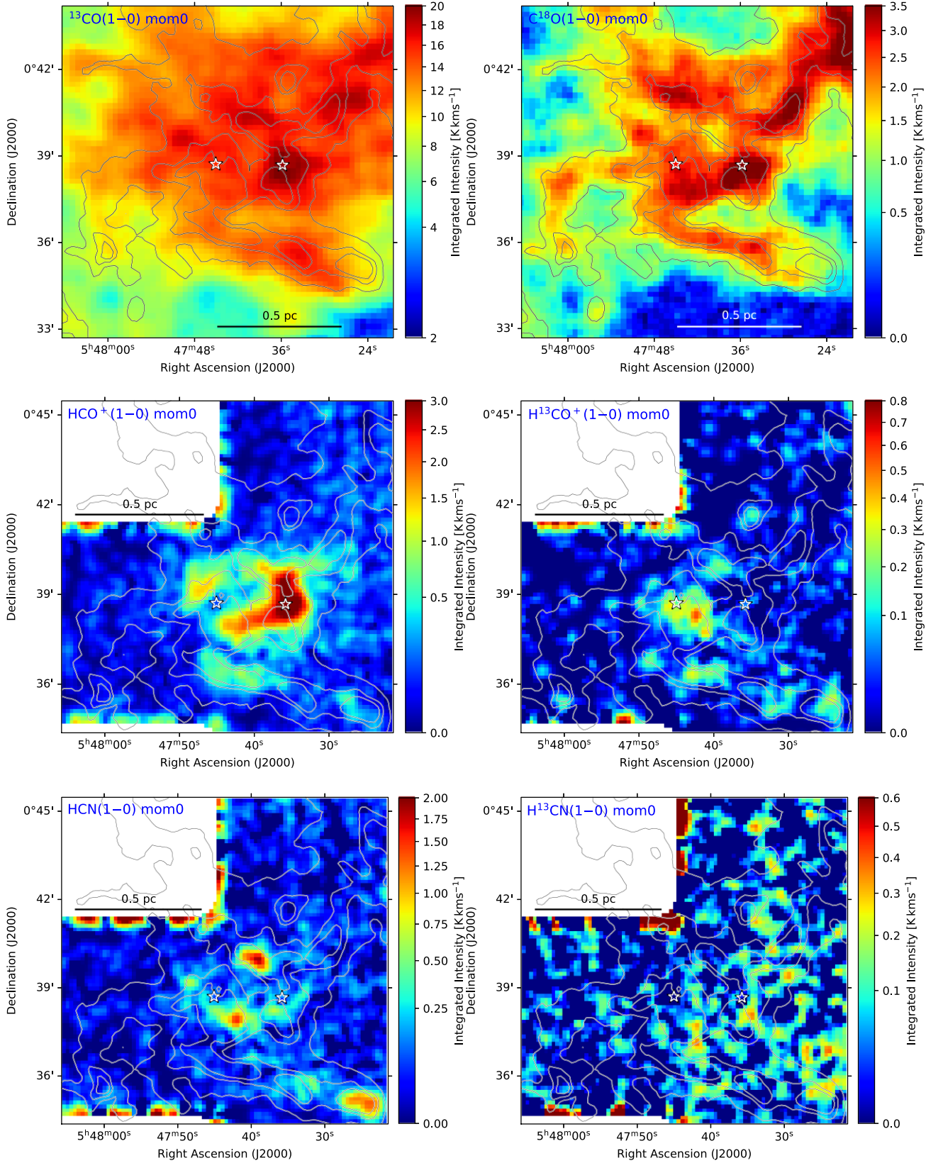
Figure B1. Integrated intensity (moment 0) maps of the hub centre (in main beam temperature) in the molecular lines indicated in the upper left-hand corner. Higher intensity ‘strings of beads’ at the map edges are artefacts. In all panels smoothed column density contours are overplotted, and the left- and right-hand white stars mark the locations of IRAS 05451+0037 and LkH \alpha 316, respectively.
