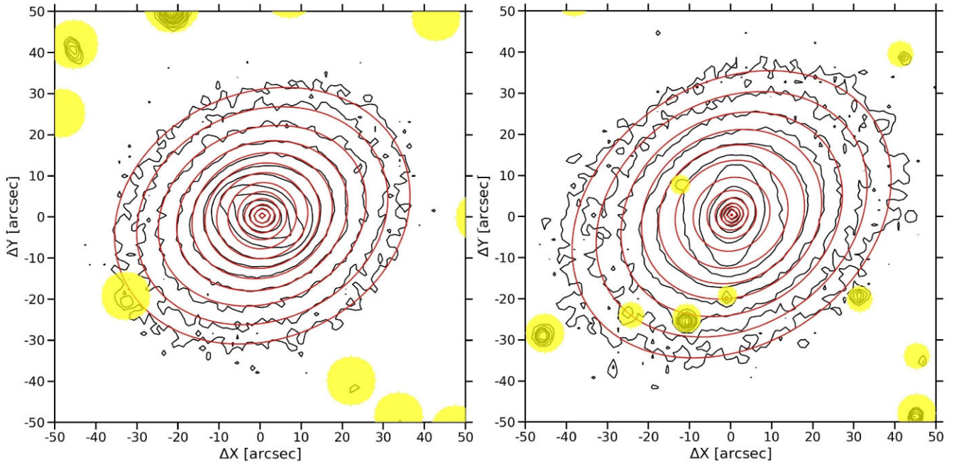
Figure 2. Some reference isophotes for the SDSS i -band image (black lines) and MGE model (red lines) of NGC 4264 (left-hand panel) and NGC 4277 (right-hand panel). The FOV is 1.7 \times 1.7 arcmin 2 and oriented with North up and East left. Flux levels are normalized to the central surface brightness of the image and the contours are spaced by 0.5 \text{ mag arcsec}^{-2} . While the MGE model was constrained using the original image, the image shown here is binned by 3 \times 3 \text{ pixels}^2 to reduce the noise for comparison purposes only. The yellow circles correspond to masked regions.
