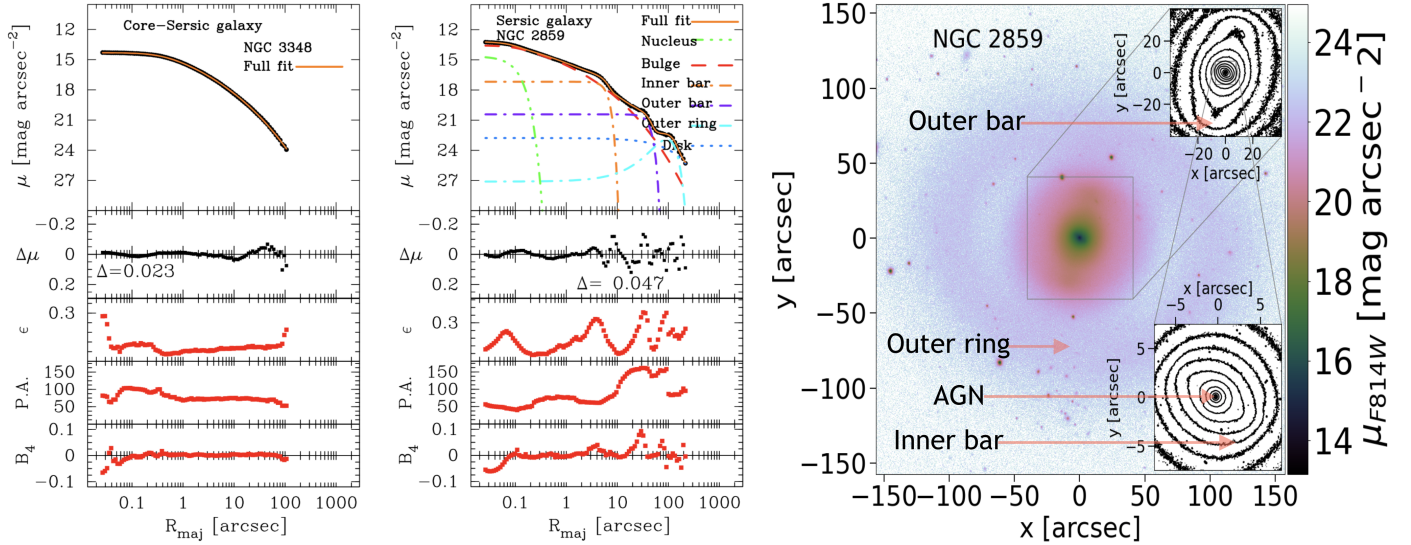
Fig. 6. Examples of fits to the major-axis surface brightness profiles of LeMMINGs galaxies. Left-hand panel: the core-Sérsic model fit to the major-axis HST WFC2 F814W-band light profile (black dots) of the elliptical LeMMINGs galaxy NGC 3348 (orange solid curve). The ellipticity ( \epsilon ), position angle (PA), and B4 profiles, along with the residual profile and rms residual ( \Delta \sim 0.023 \text{ mag arcsec}^{-2} ) for this massive core-Sérsic galaxy are also shown. Middle panel: composite (HST ACS+SDSS), F814W-band surface brightness, \epsilon , PA, and B4 profiles of the doubled-barred lenticular LeMMINGs galaxy NGC 2859. The SDSS i -band data are zero-pointed to the HST F814W-band profile. Six-component decomposition of the galaxy major-axis surface brightness profile (black dots) into a nuclear component, a bulge, an inner bar, and three outer galaxy components (bar+ring+disc) are denoted by various broken curves which are summed up to the final model (orange solid curve) that describes the galaxy. The stellar light distribution of the nuclear component (which we tentatively identify as AGN, see Baldi et al. 2018, 2021a) is modelled with a two-parameter Gaussian function and dominated by the Sérsic ( n \sim 3.6 ) bulge. The inner and outer bars are described using two Sérsic models each with n \sim 0.2 . The outer, extended exponential disc is the dotted blue curve. The three-parameter Gaussian ring model (cyan dot-dashed curve) describes the outer ring. The two bars and the large-scale ring are accompanied by three local maxima in \epsilon and B_4 and twists in PA. Each model component is convolved with a Gaussian PSF. The residual profile along with the small rms residual \Delta \sim 0.047 \text{ mag arcsec}^{-2} . We fit six model components which are summed up to a full model with 16 free parameters. Right-hand panel: SDSS image of NGC 2859. The top and bottom insets show the surface brightness contours of the galaxy's SDSS and HST ACS images, respectively. North is up and east is to the left.
